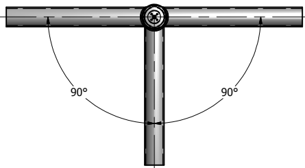
VIEW A-A SB-39 TOP VIEW DETAIL
